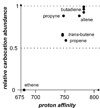
Figure 1. Relative carbocation abundance I_{\text{rel}} = I(\text{carbocation})/[I(\text{carbocation}) + I(\text{VO}_3\text{H}_2^+)] vs. proton affinities [20] (in \text{kJ mol}^{-1} ) of the produced alkenes in the reactions of \text{VO}_2^+ with alcohols.
